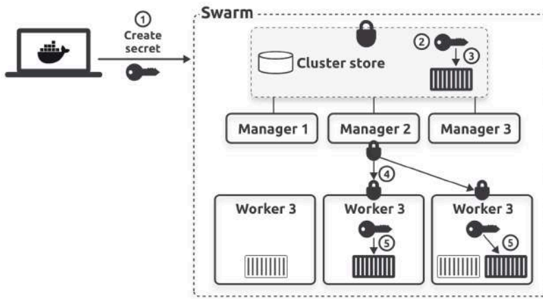
Figure 16.10 - Secret workflow
