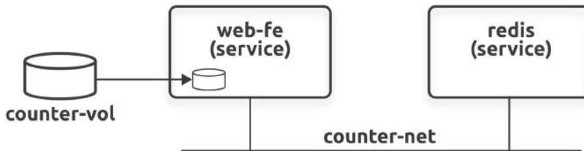
Figure9.1 - Sample app
