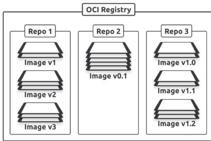
Figure 6.3 - Registry architecture
