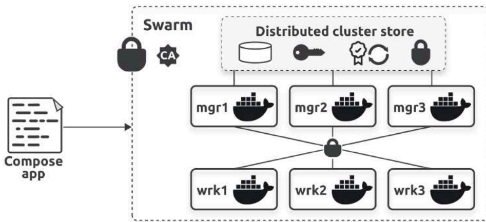
Figure 10.1 High-level swarm
